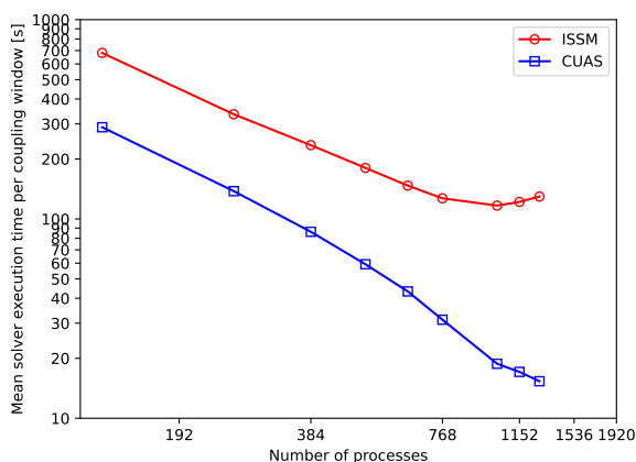
Figure 12. Average execution time required by the CUAS and ISSM solver during one coupling window for CUAS and ISSM for different numbers of MPI processes.
