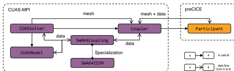
Figure 4. Structure of the CUAS-preCICE adapter. The coupling is integrated into and coordinated by the existing CUASolver , but most of the coupling logic is isolated in added classes. The coupling data that is read and written flows through a utility class (specialized for coupling with ISSM) that handles transformations such as deriving ice pressure and transforming units.
